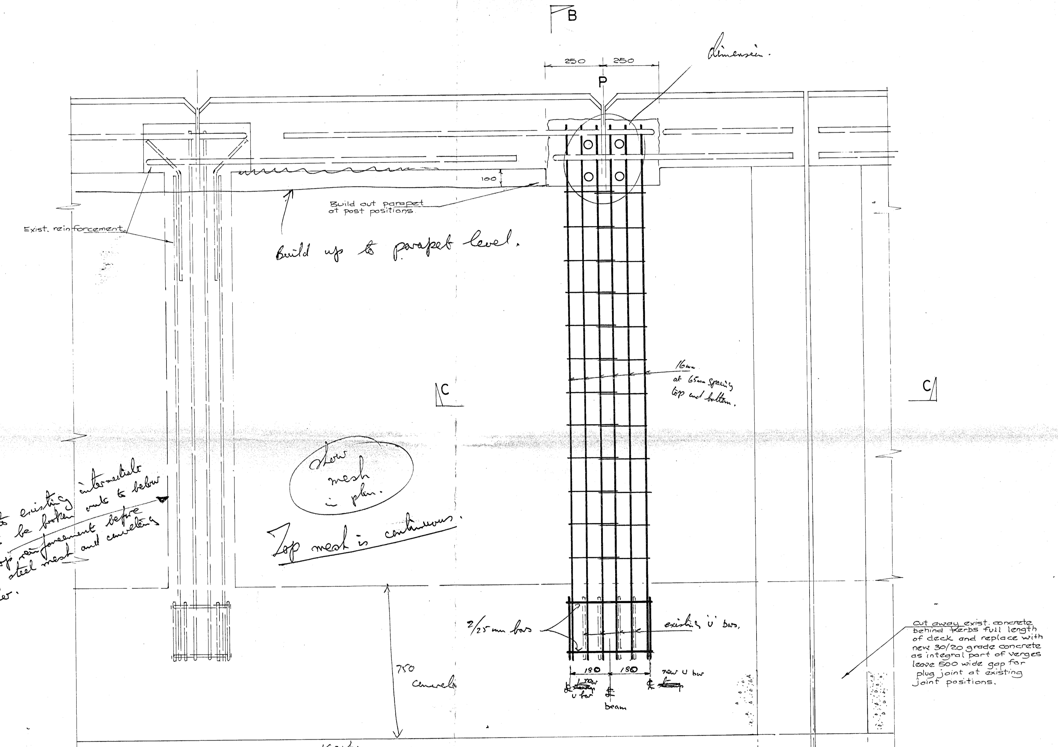
DETAIL OF KERB MODIFICATION OVER JOINTS. SCALE 1:10
