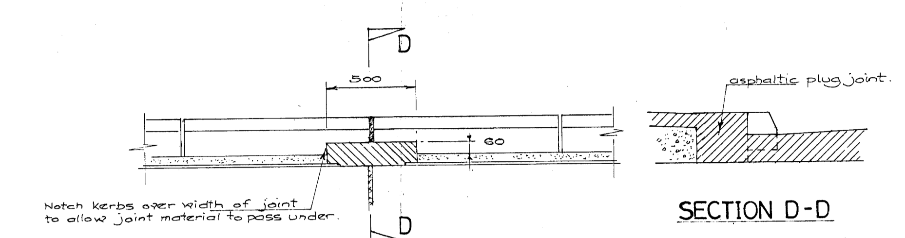
DETAIL OF KERB MODIFICATION OVER JOINTS. SCALE 1:10
